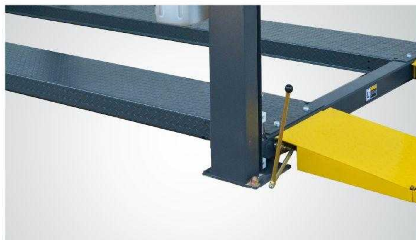
▲ Patented concealed safety lock control device with single-point manual lock release.
